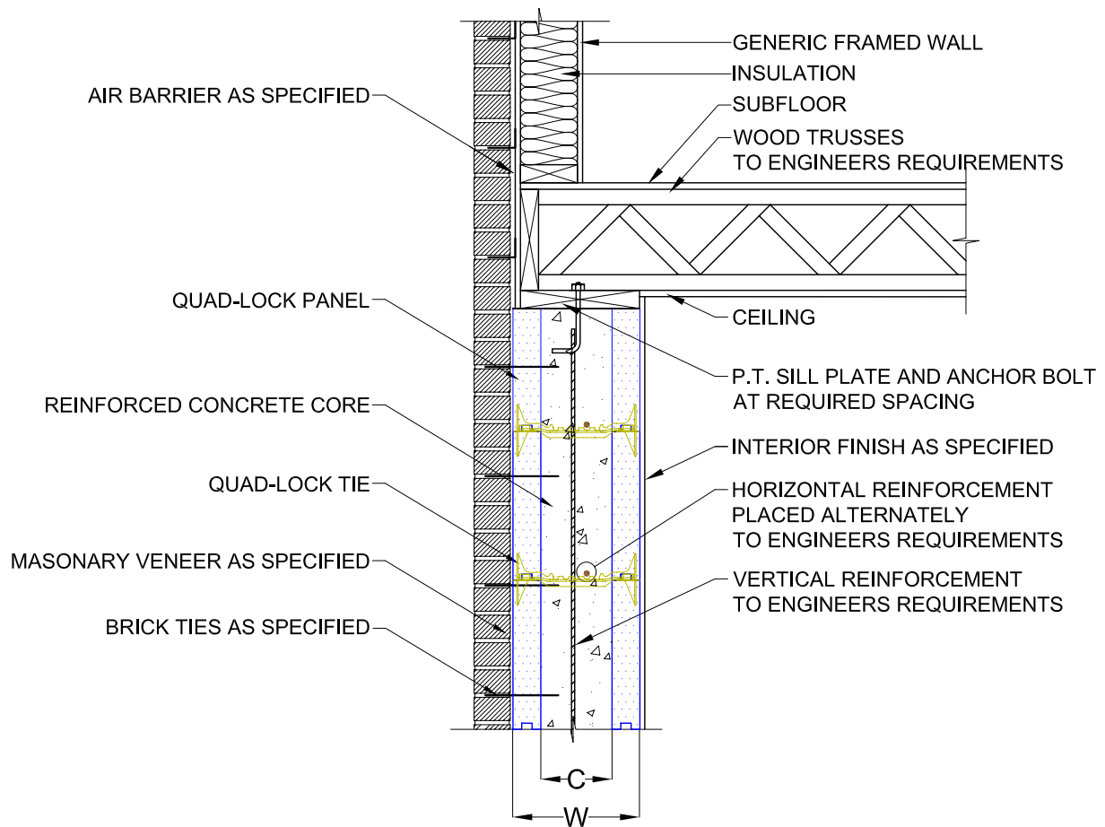
1 2.5 SECTION DETAIL
