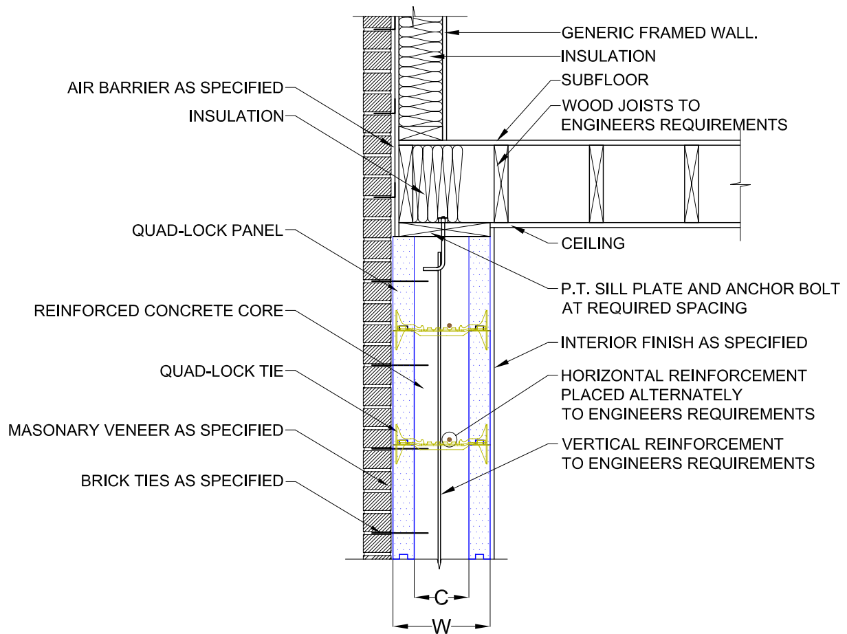
1 SECTION DETAIL 2.2
